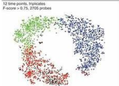
Figure3_tSNE_SelfOrganization
